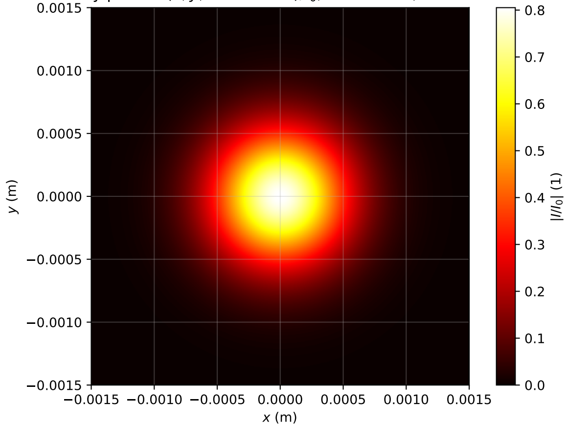
Intensity profile I(x, y, z = 1.274m)/I_0 , Pin=0.2Pcr, artificial time
